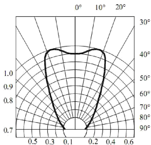
RADIATION DIAGRAM
