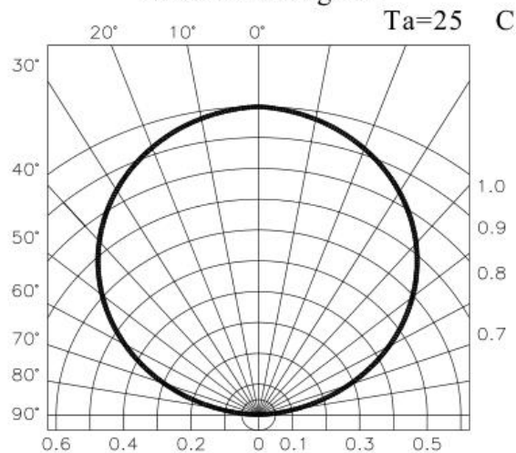
Radiation Diagram
